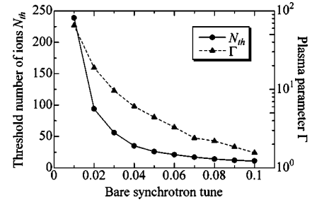
FIG. 9. Threshold number of ions in a bunch and the corresponding plasma parameter vs bare synchrotron tune. The lattice parameters are identical to those in the case of Fig. 1.
