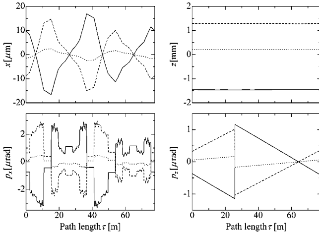
FIG. 2. Single-particle orbits in a bunched string crystalline beam. The trajectories of three ^{24}\text{Mg}^+ ions arbitrarily selected from the beam in Fig. 1 have been plotted.
