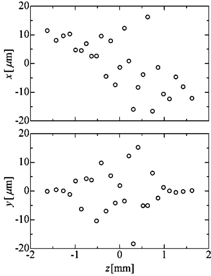
FIG. 8. Spatial configuration of a bunched beam cooled by the linear dissipative force with f_x=f_y=0.01 and f_z=0.33 . Other parameters are identical to those in the case of Fig. 1.
